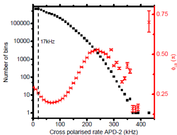
Figure 2.(black) Histogram of the number of photons scattered into cross-polarized channel in 100ms bins: high counts indicate that the QD is on resonance. (red) Phase shift determined as a function of count rate, reaching >0.5\pi .
