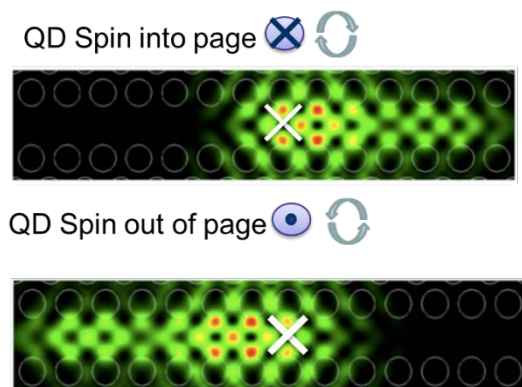
Figure 1. Finite-difference time-domain simulation of circular dipole emission at a polarization singularity. showing unidirectional emission whose direction depends on dipole helicity.
